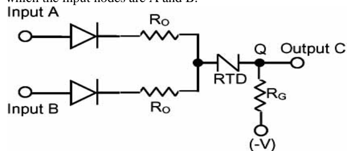
Fig-4.4: Circuit diagram of the diode logic XOR gate using the molecular RTD
