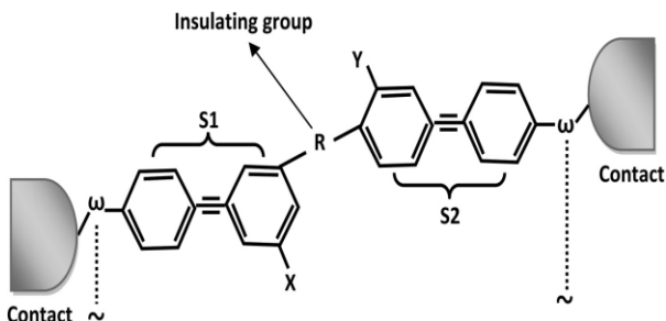
Fig-3.3: Structure of a molecular diode
