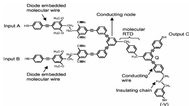
Fig-4.5: Schematic representation of the diode logic molecular XOR gate using the molecular RTD
