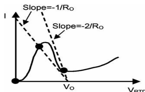
Fig-4.6: Current-voltage characteristics of an RTD incorporated into the molecular XOR gate
