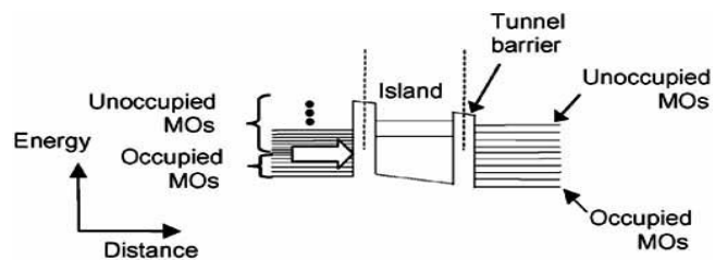
Fig-3.6: Band diagram of the molecular RTD showing the 'OFF' state
