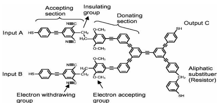
Fig-4.3: Schematic of the exemplary poly-phenylene diode logic molecular AND gate
