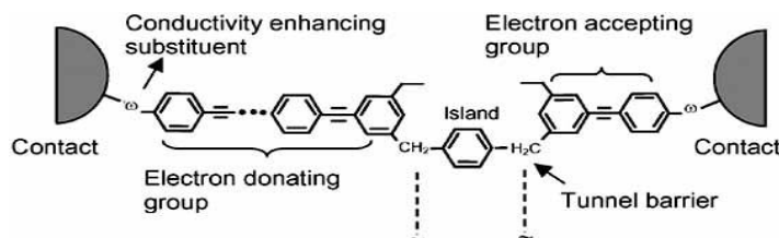
Fig-3.5: Structure of molecular resonant tunneling diode
