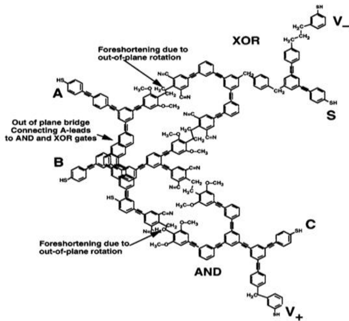
Fig-5.2: Molecular Electronic Half Adder CONCLUSION
