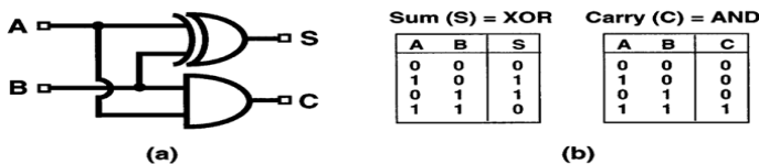
Fig-5.1: Binary Half Adder
