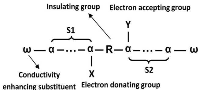
Fig-3.4: Schematic representation of a molecular diode
