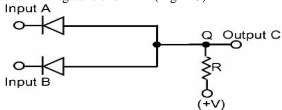
Fig-4.1. Circuit diagram of the diode logic AND gate
