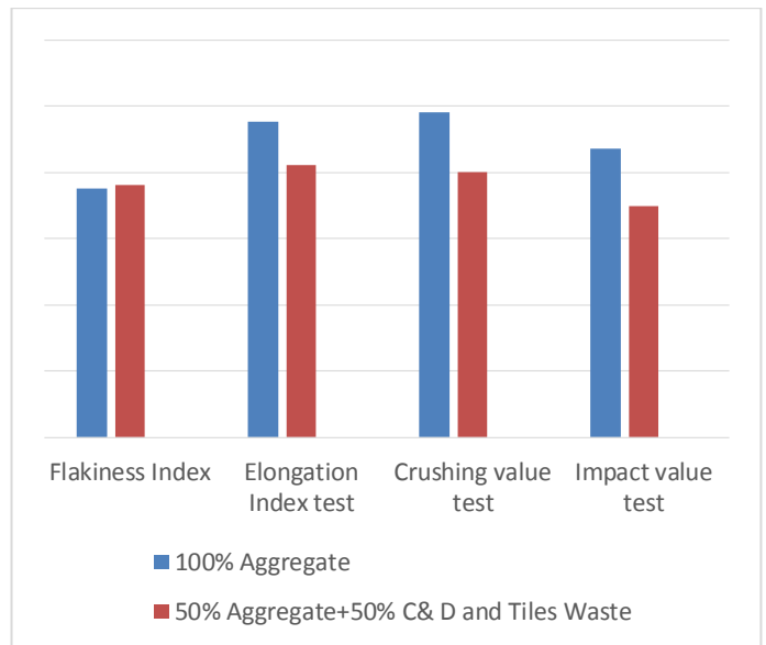
Fig.3:-Comparison of conventional and mixed aggregate
