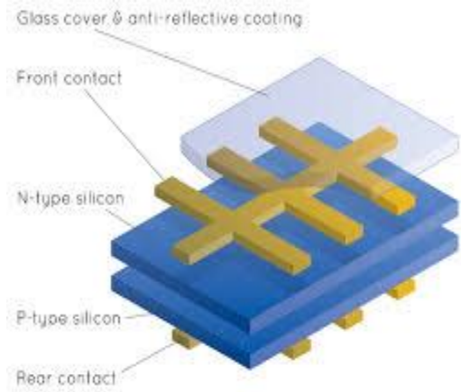
Figure 2. Conventional solar cell
