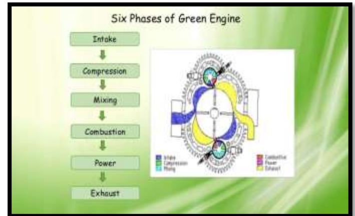
Figure No. 3: 6 PHASES OF GREEN ENGINE
